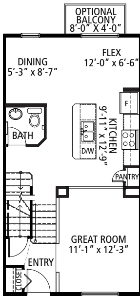
MAIN FLOOR STANDARD 612 sq. ft.
