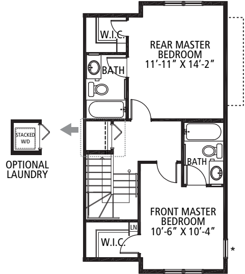
UPPER FLOOR OPTION DUAL MASTERS WITH ENSUITES 591 sq. ft.
